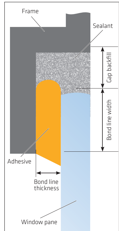
Fig. 2 Bonding a decorative panel vertically
